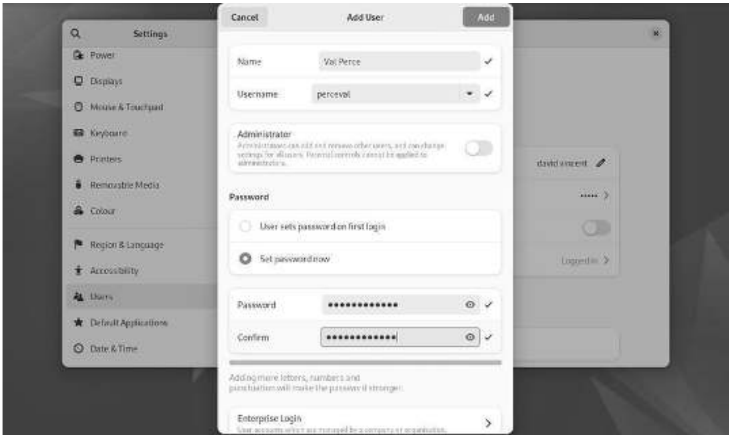
User configuration
