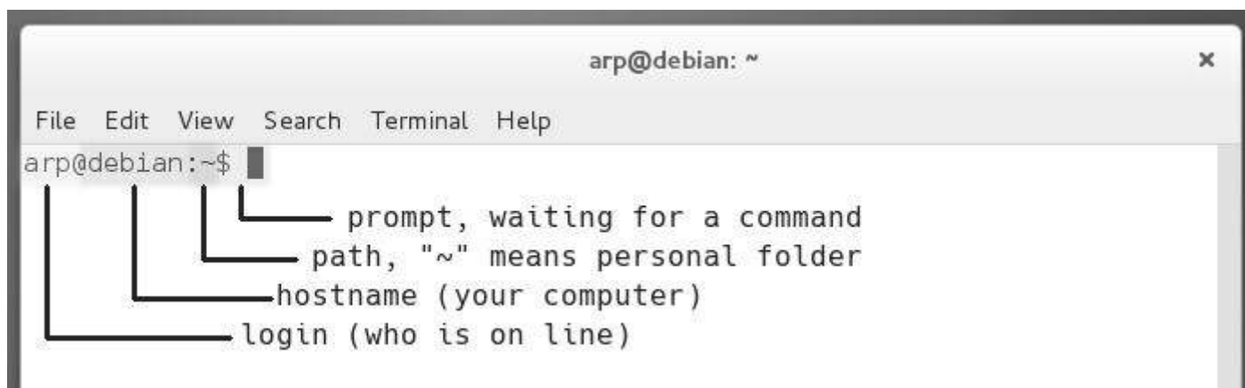
Terminal presentation
