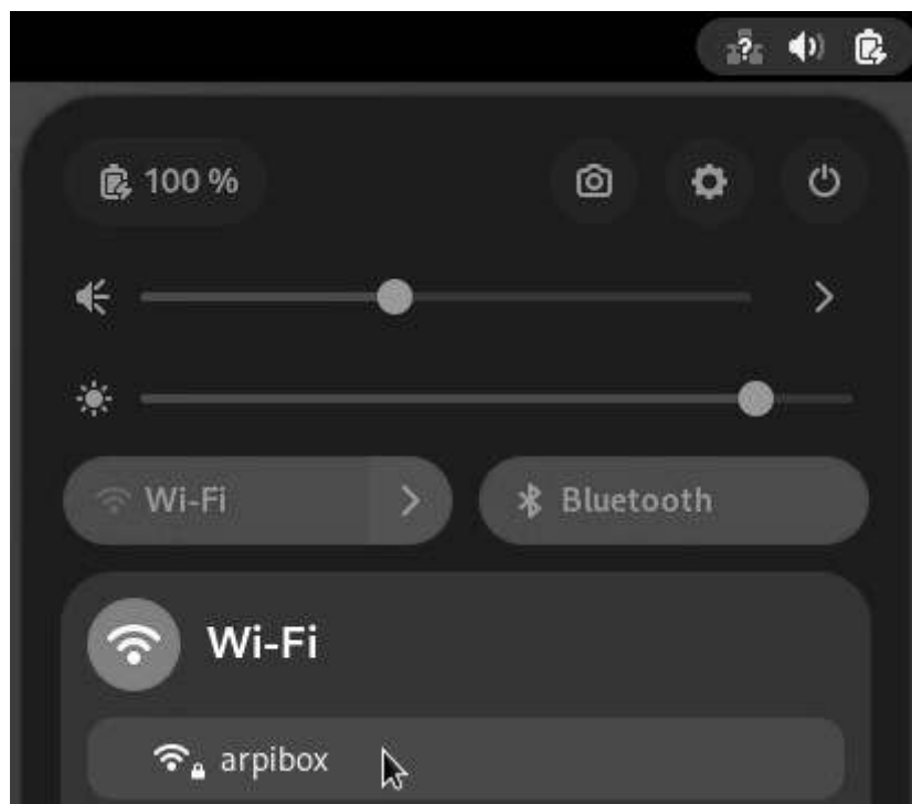
Network selection
