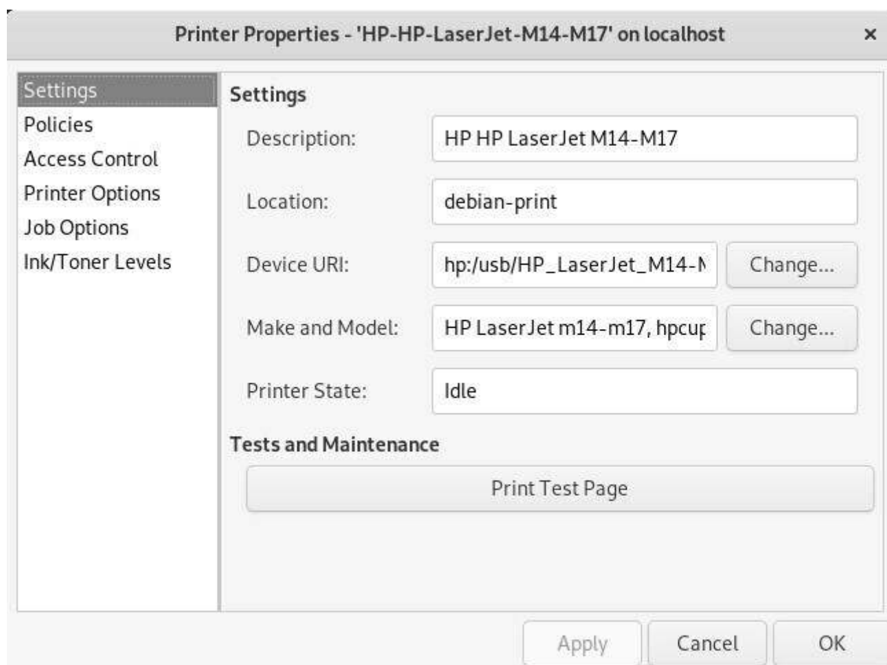
Printer configuration
